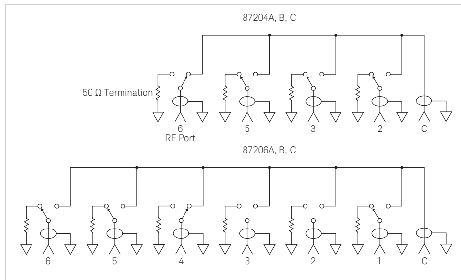
Figure 1. Keysight 87204A/B/C and 87206A/B/C simplified schematics
