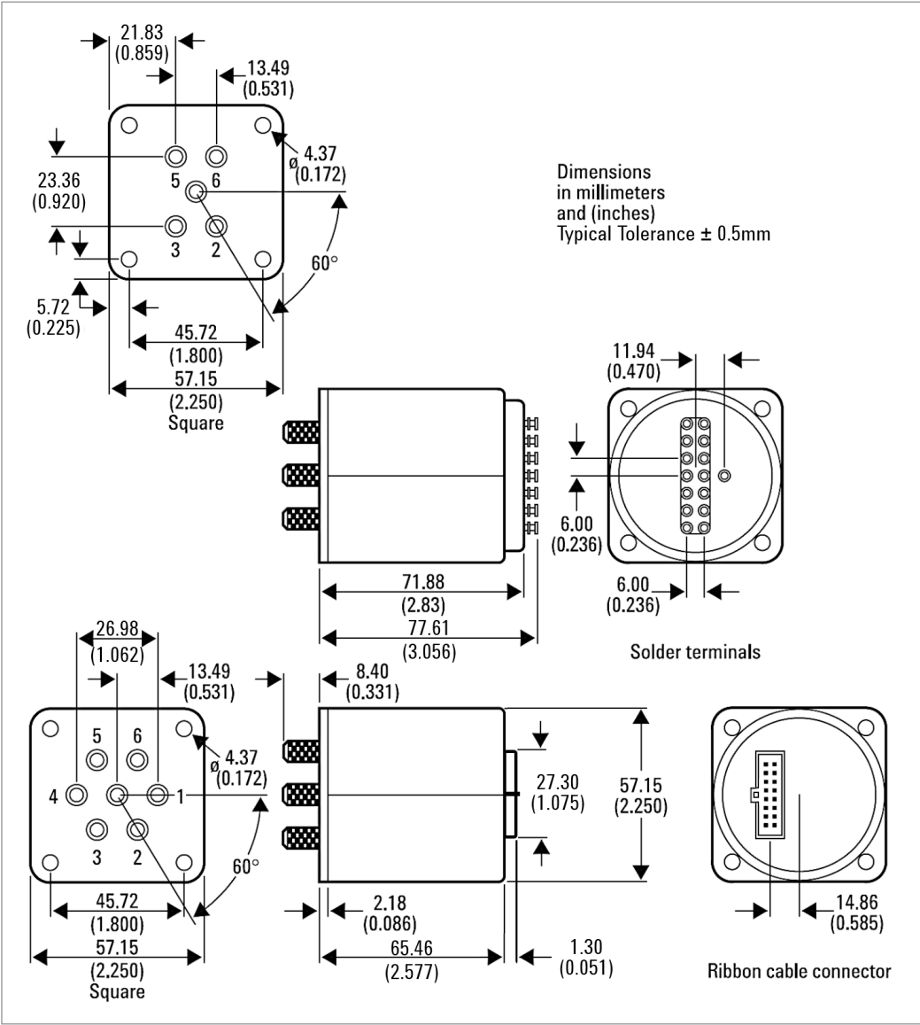
Figure 9. Product outlines
