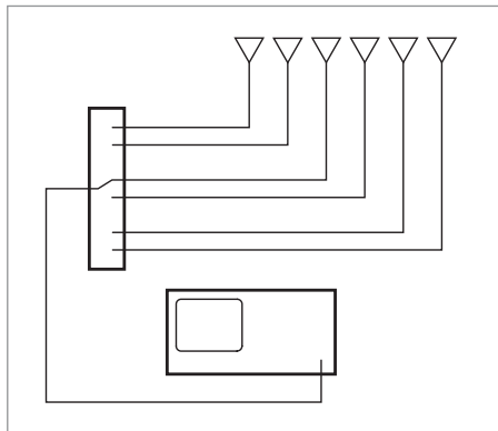
Figure 3. Multiport matrix
