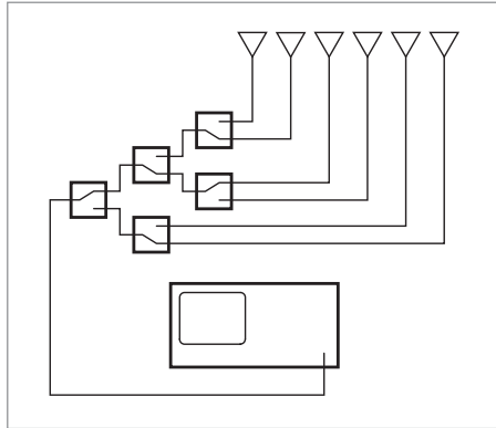
Figure 2. Tree matrix
