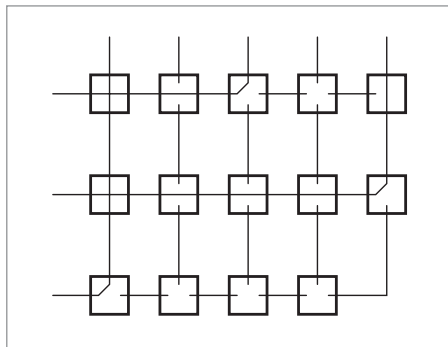
Figure 4. Cross-point matrix
