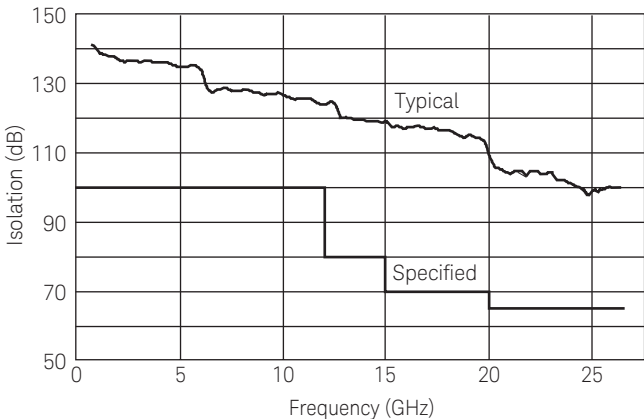
Figure 7. Isolation
